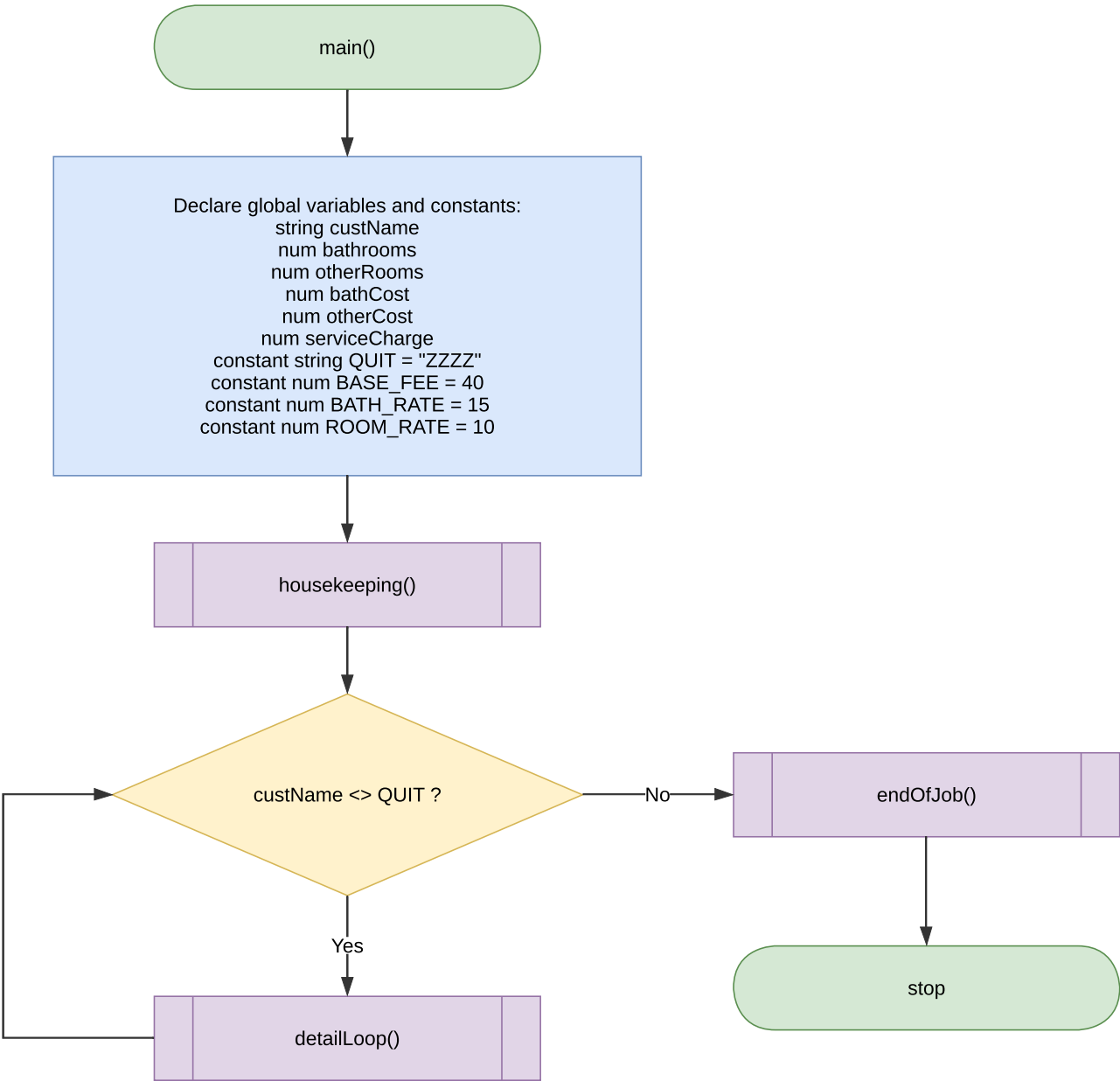
Main Program
